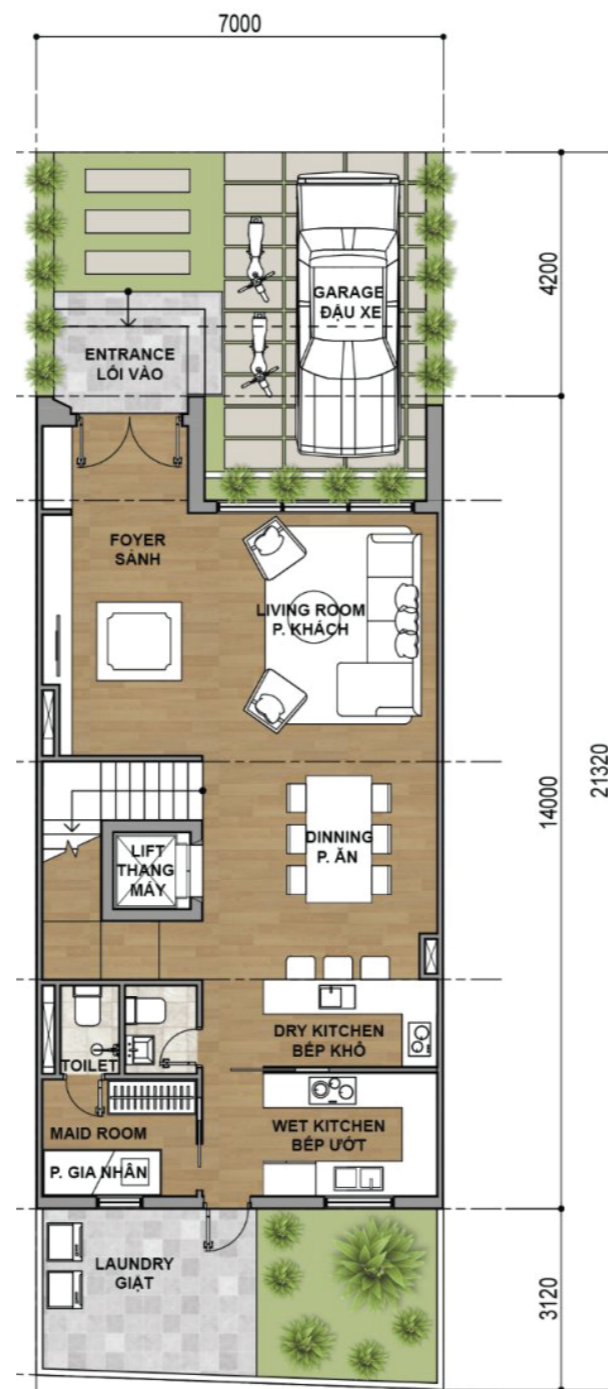
1 1ST FLOOR PLAN MẶT BẰNG TẦNG 1
