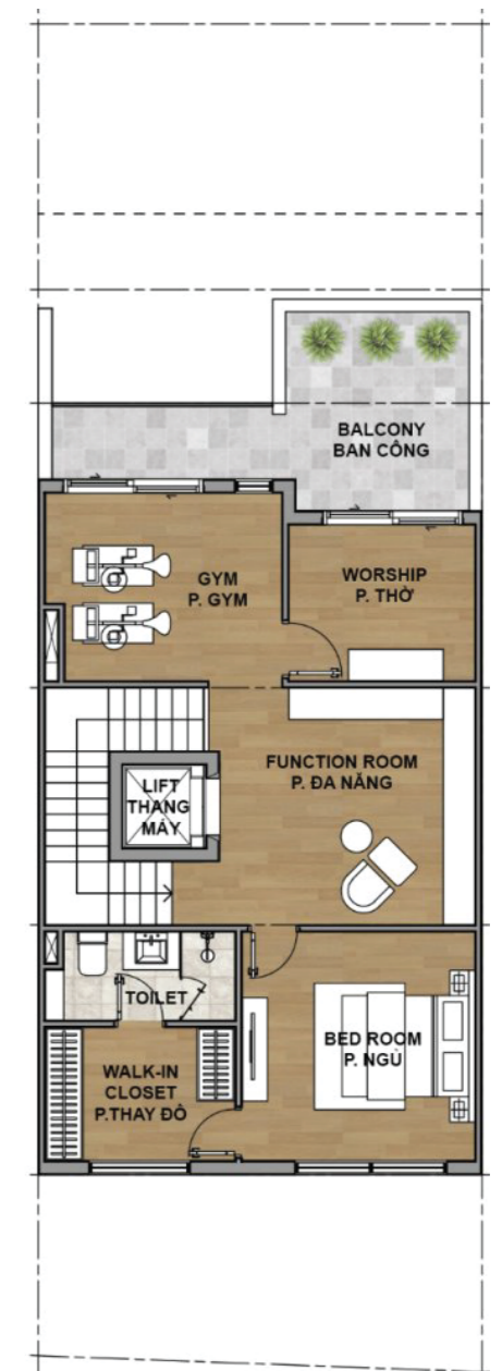
4 4TH FLOOR PLAN MẶT BẰNG TẦNG 4
